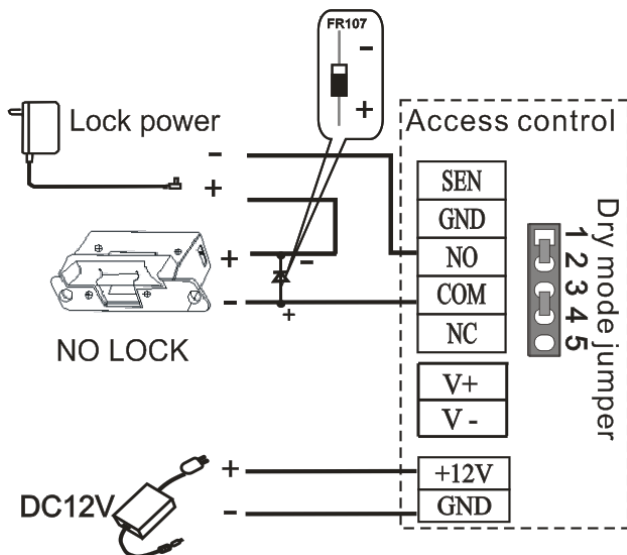
4. Dry mode: External power supply for NC Lock
