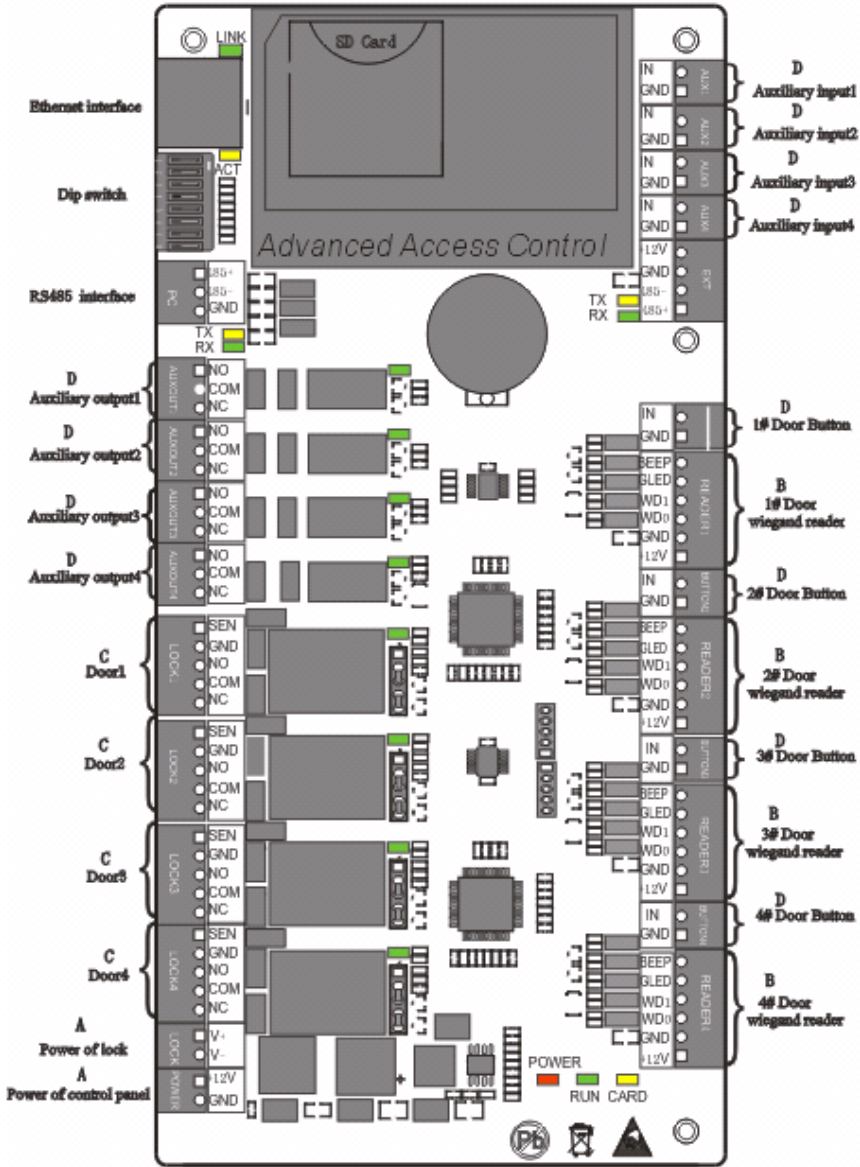
C3-400 terminal connection diagram
