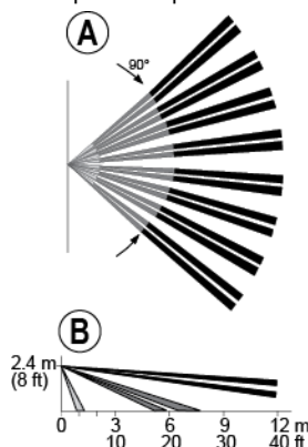
Figure 6. Coverage Pattern
