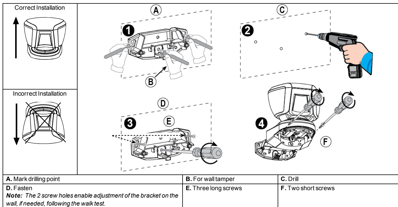
Figure 2 - Installation
