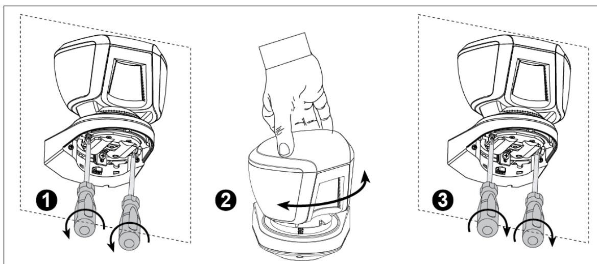
Figure 2 - Installation
