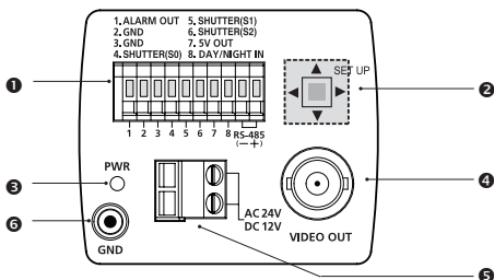
<AC24V/DC12V (SCB-2001(P))>
