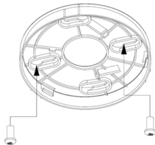
Fig. 5 – Fixing base
